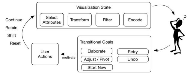
Fig. 11. Conversational transitions model [242] that describes how to transition a visualization state during an analytical conversation.
