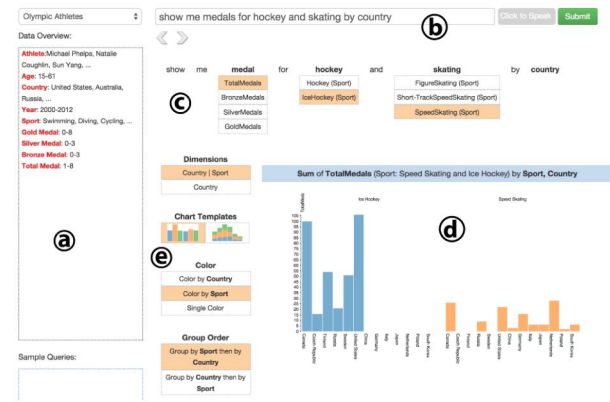
Fig. 7. Ambiguity widgets in Datatone [63]. The user can correct the imprecise system decisions caused by ambiguity.
