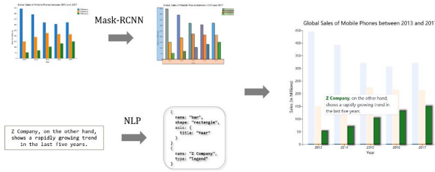
Fig. 12. Visualizations with annotations generated by Vis-Annotator [122].
